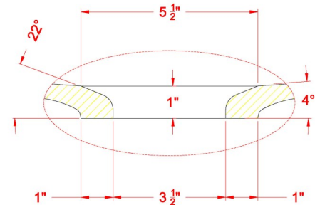
Drain Detail
