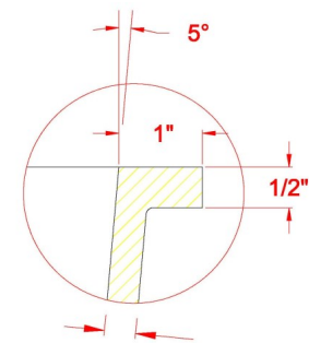
Flange Detail
