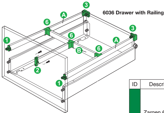
Front partition clip Screw-on
