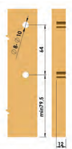
• Assembly measurements for dowel in front
