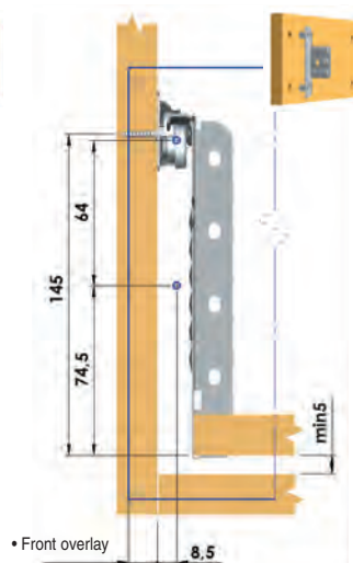
• Front overlay • Assembly measurements for screw-on front
