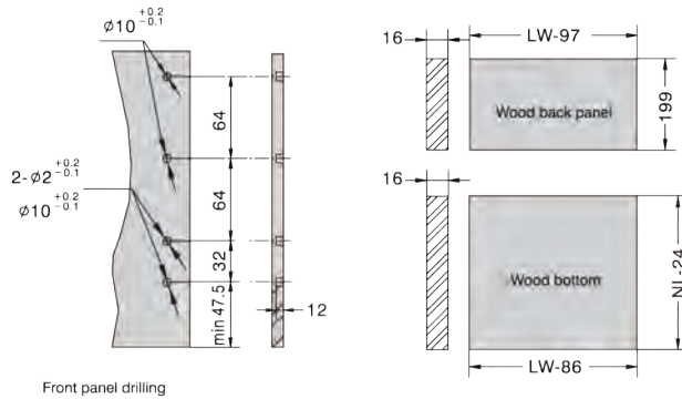
Front panel drilling
