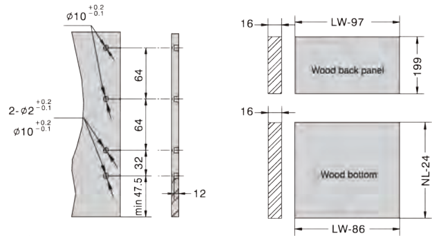
Drawer front Dimensions
