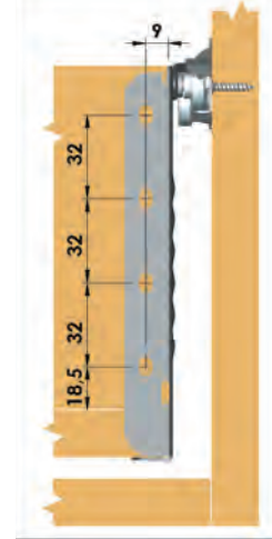
• Drawer back panel drilling measurements
