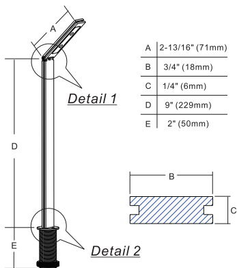
9" SPLENDOR 6 WATT HIGH POWER LED Item No. H5.12117
