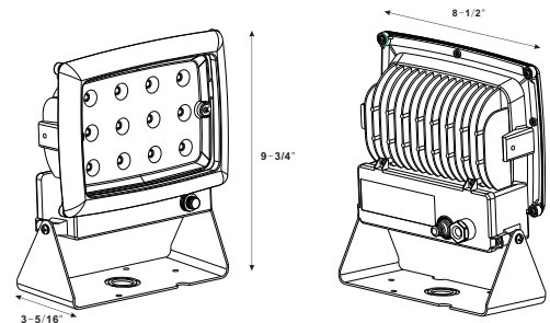
Details: LED-012F-BZ-110V
