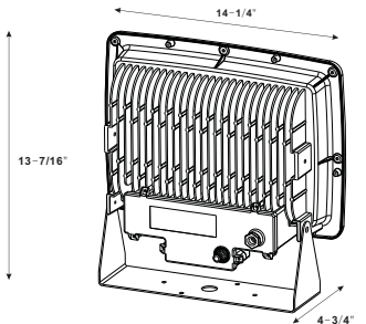
Details: LED-120F-BZ-110V, LED-120F-W-110V
