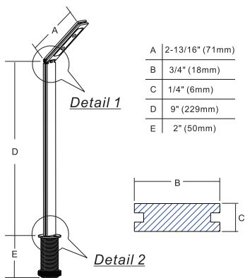
9" SPLENDOR 6 WATT HIGH POWER LED Item No. H5.12115
