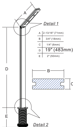
19" SPLENDOR 6 WATT HIGH POWER LED Item No. H5.12116
