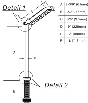
9" RADIANCE 3 WATT HIGH POWER LED Item No. H5.12111
