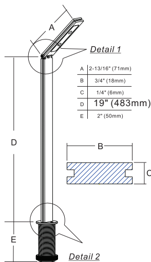
19" SPLENDOR 6 WATT HIGH POWER LED Item No. H5.12118
