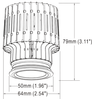
H5.94015 LED ENGINE LIGHT (Without Trim Ring)
