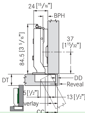
Drawings Show Tiomos With Base Plate, Height 02.
