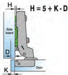
HALF OVERLAY HINGE 14-104
