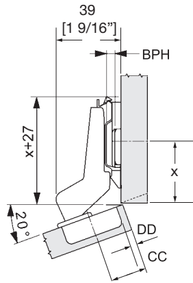
Nexis Self-closing Screw-on .....12-762 Nexis Impresso Self-closing .....12-765
