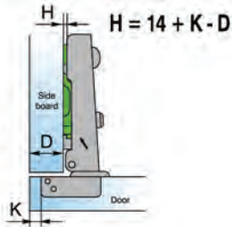
FULL OVERLAY HINGE 14-100
