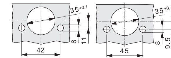
Drawings Show Tiomos With Base Plate, Height 02.
