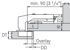
Drawing shows Tiomos with a base plate height (BPH) 03.
