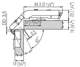
19mm door thickness with base plate height 0
