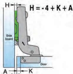
INSET OVERLAY HINGE 14-108
