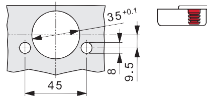
Drawings show mounting plate, thickness 02.
