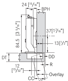
Drawings Show Tiomos With Base Plate, Height 02.
