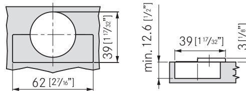
Drawings Show Tiomos With Base Plate, Height 02.
